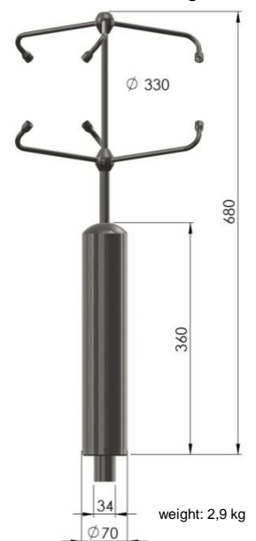
Mechanical drawing
